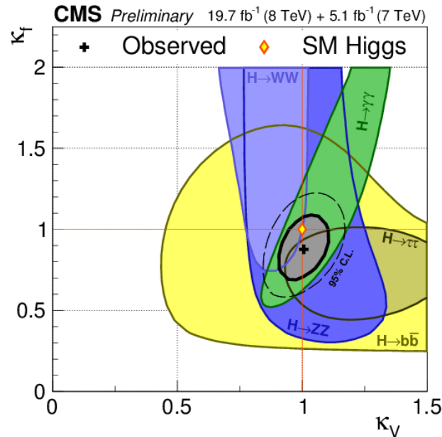
Figure 2: Compatibility of Higgs boson couplings to vector bosons ( V ) and fermions ( f ) with the standard model expectation (diamond). The allowed regions by each group of decay modes analyzed (colored) combine into a much smaller region (grey) that is fully compatible with the standard model.
