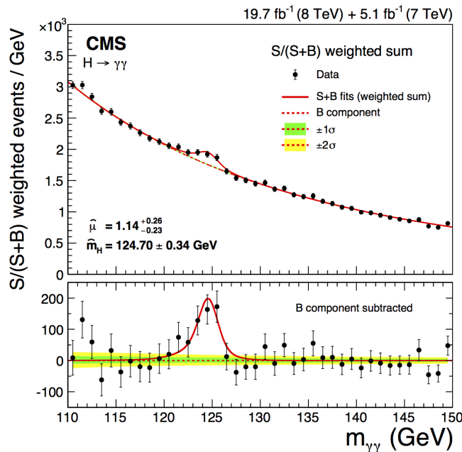
Figure 1: Combined two-photon mass spectrum illustrating the significance of the observed excess, where events are weighted by the expected signal-to-background ratio. The corresponding background-subtracted distribution is shown in the lower panel.
